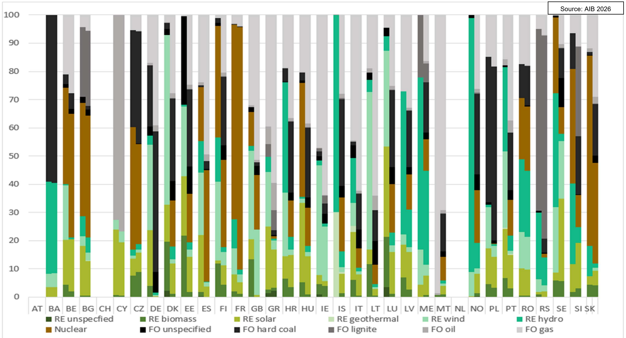
Figure 10 Production Mix (left) and <Final Residual Mix (right) 2025 (detailed fuel categories)
