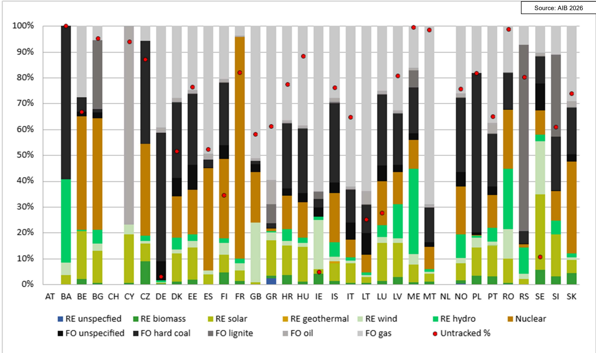
Figure 2 Residual Mixes 2025 (detailed fuel categories)
