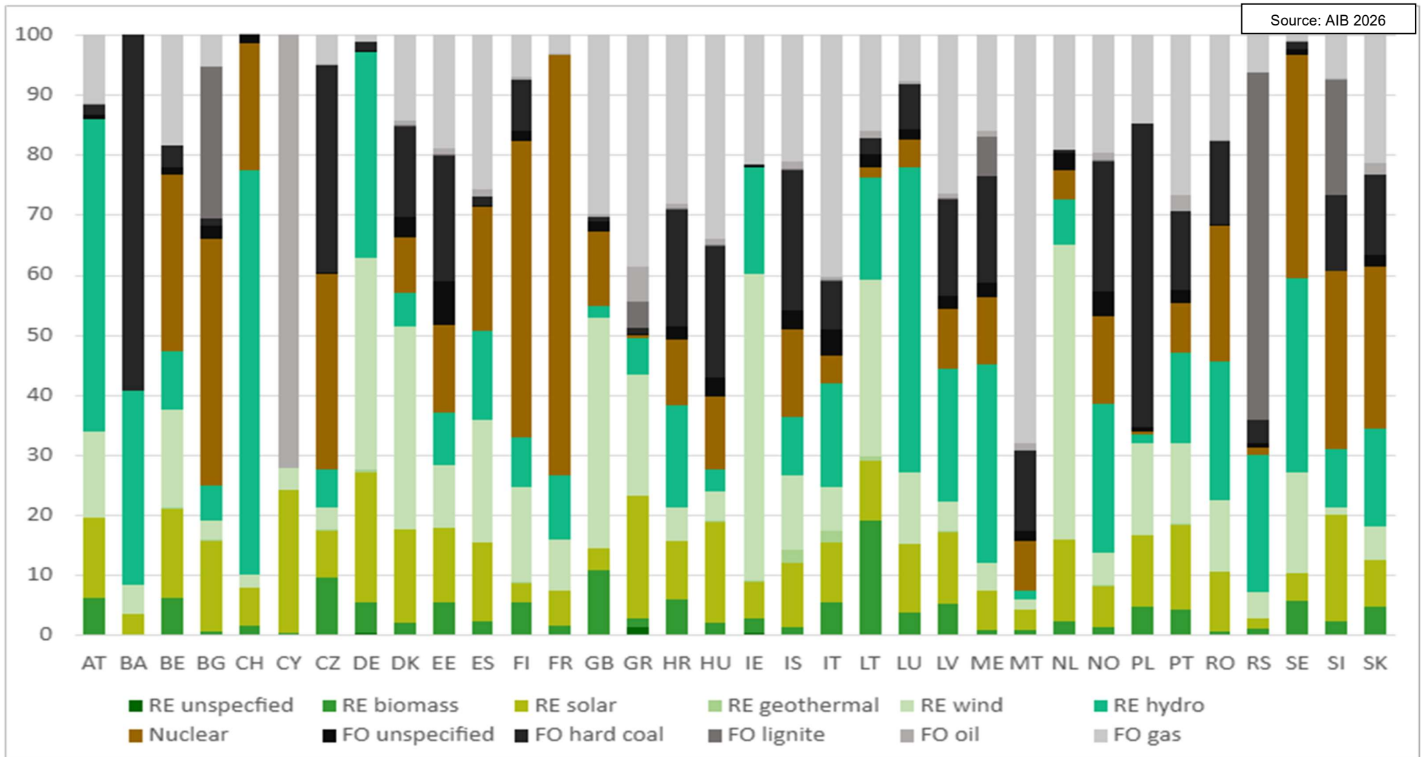
Figure 8 Total Supplier Mix 2025 (detailed fuel categories)
