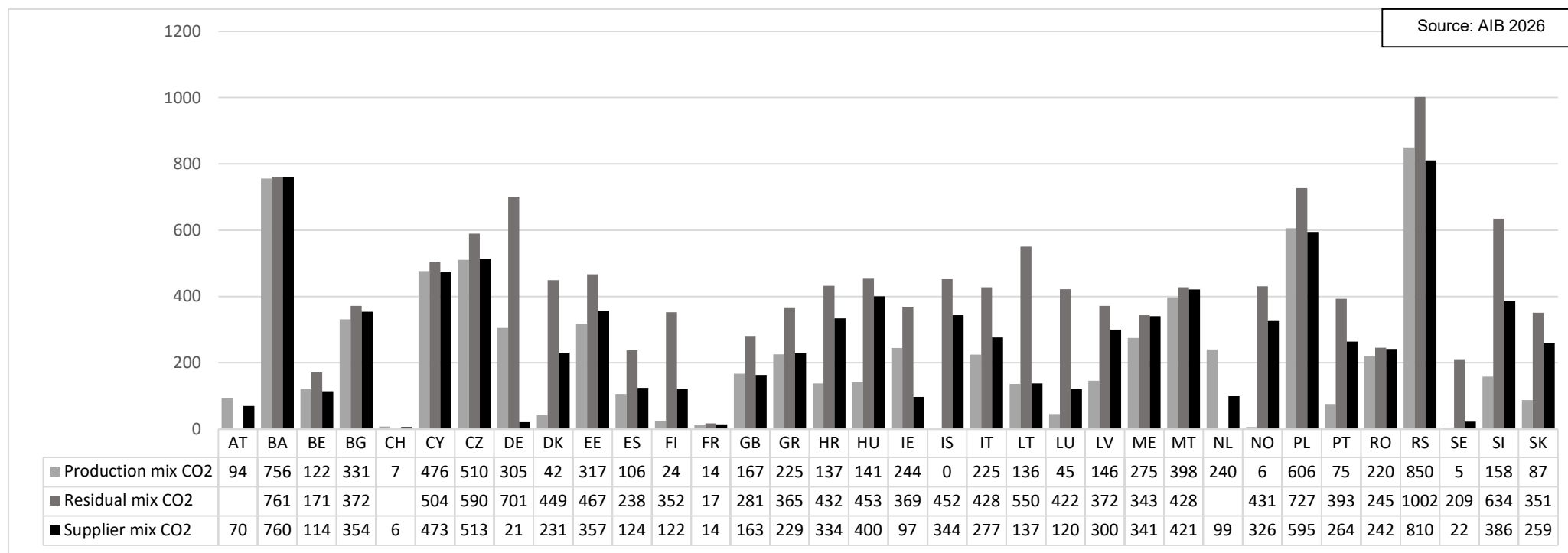
Figure 5 Direct CO2 content in Production, Residual and Total Supplier mix 2025 [gCO2/kWh]
