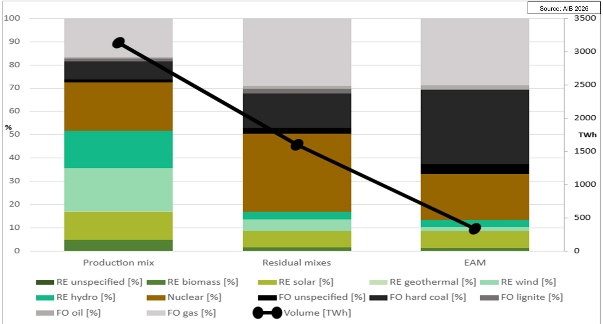
Figure 11 European Total Production Mix (left), Attributes in Final Residual Mixes (middle) and EAM (right) 2025
