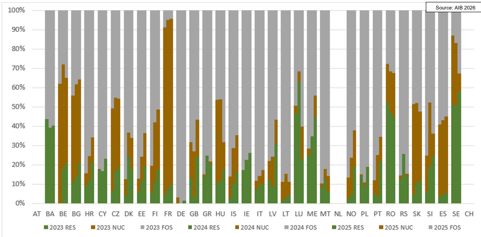
Figure 16 Residual Mixes 2023, 2024 and 2025
